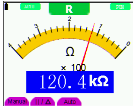
Figure 21: Resistance Measurement
